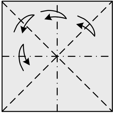
Frog base
