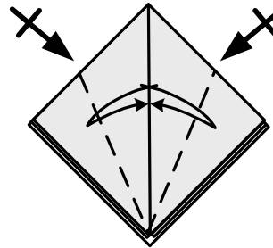
Bird base
