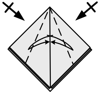
Frog base
