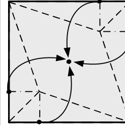
Fish base
