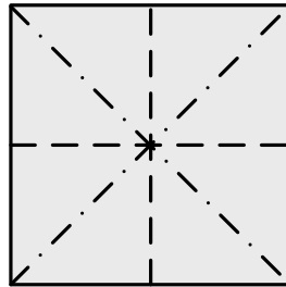
Waterbomb base
